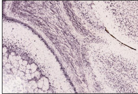
ISH: Raptor
