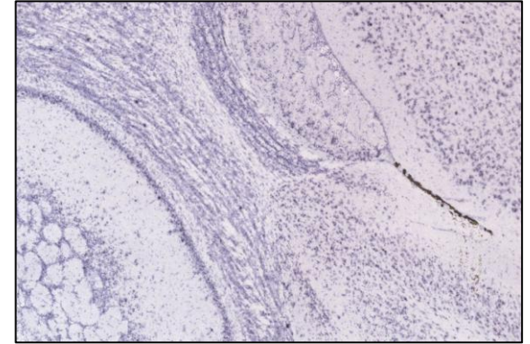
ISH: Rictor
