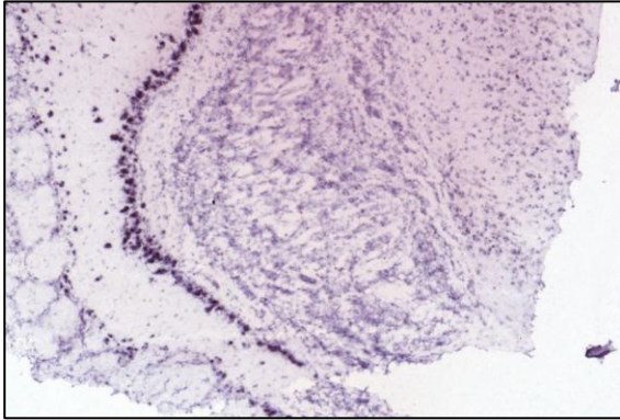
ISH: mTOR
