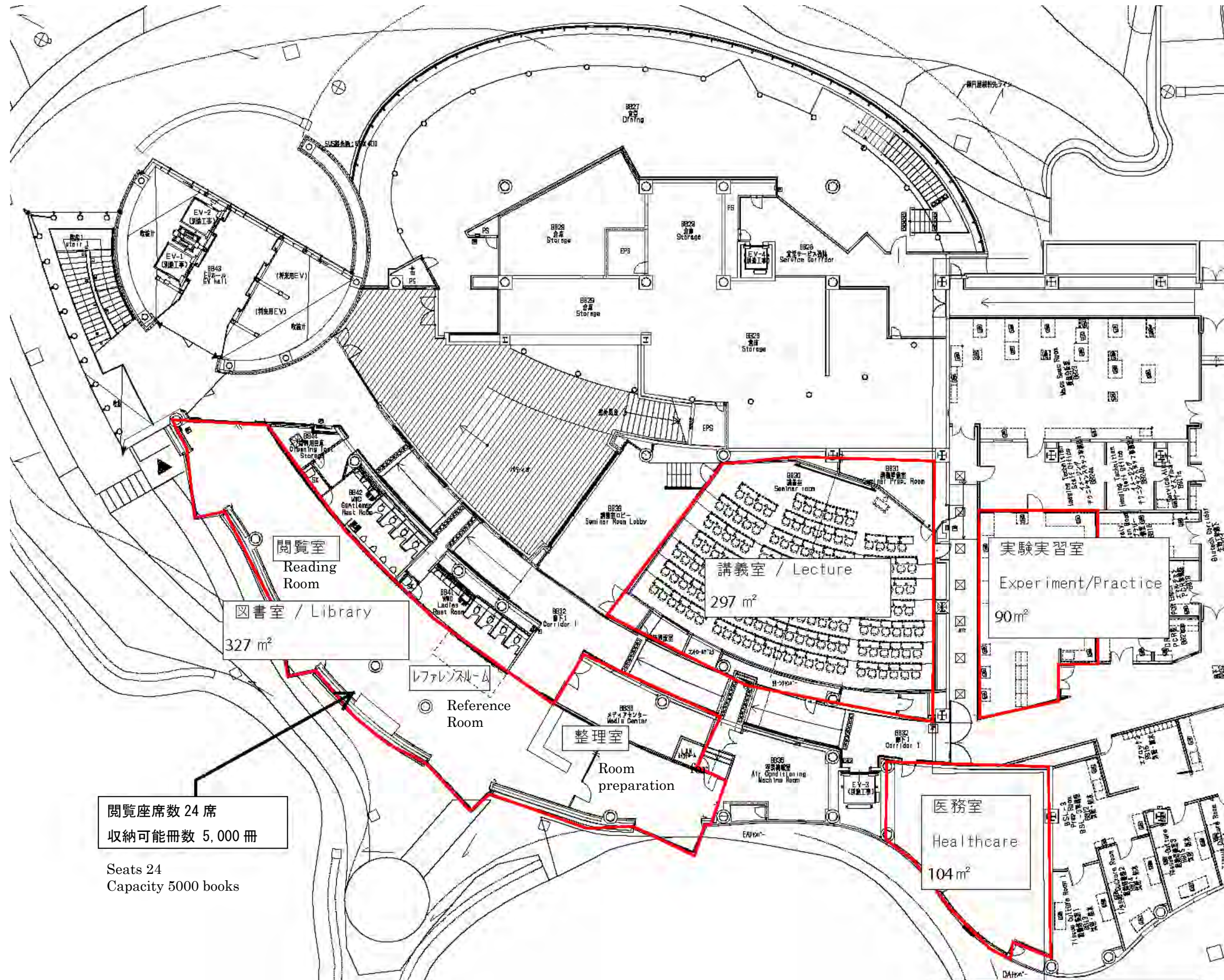
Figure showing floor plans of university buildings<B floor, Center Building>
