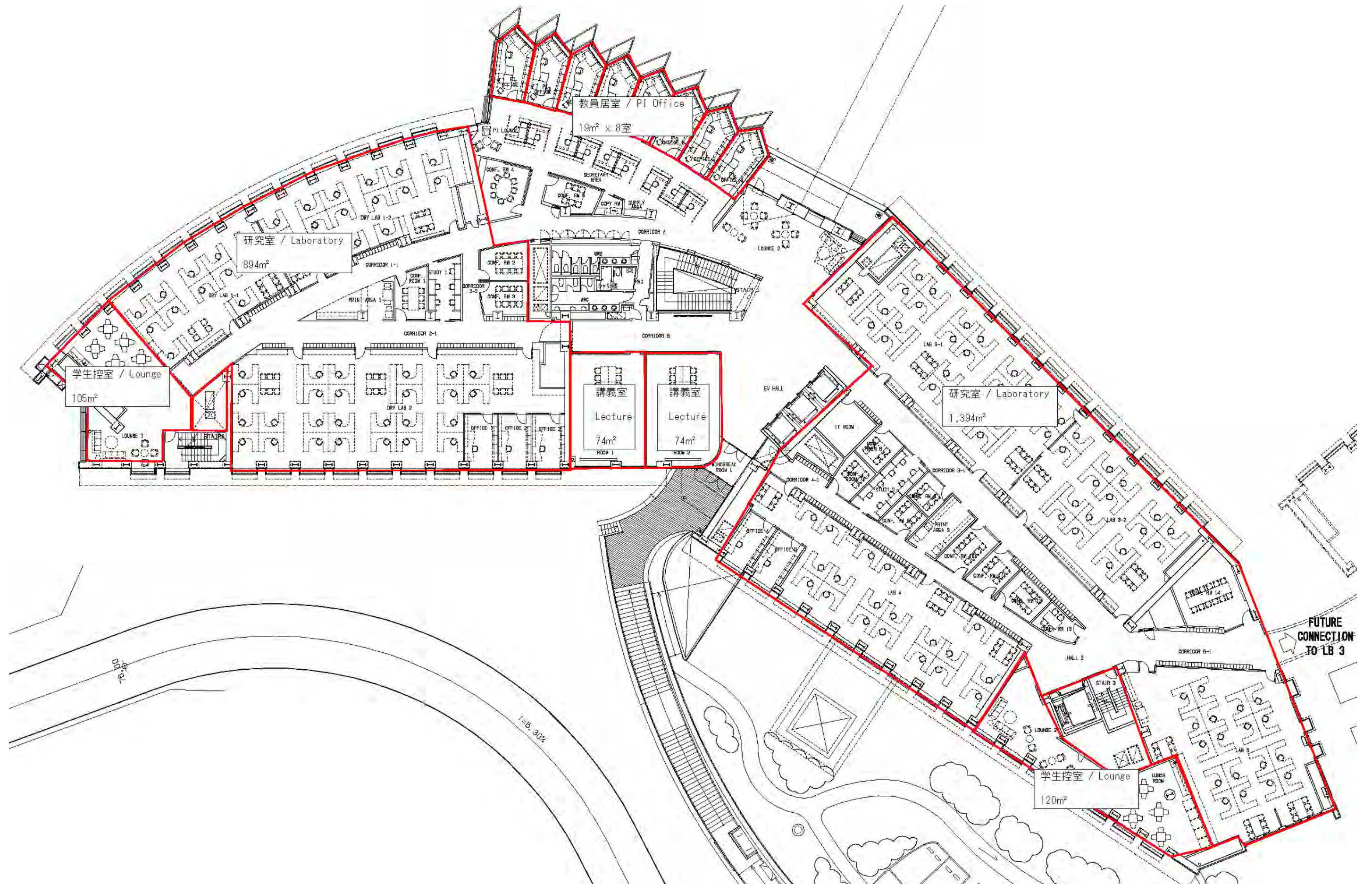
Figure showing floor plans of university buildings <B floor, Lab 2>
