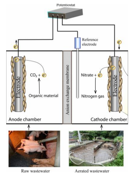
Figure 1. The novel system was created from polyacrylic reactors containing two chambers, which were separated by an ion-exchange membrane and equipped with three
