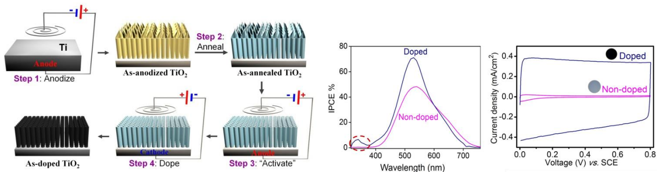
Figure 3. Electrochemical doping of anatase \text{TiO}_2 for high-performance photocatalysts and supercapacitors.
