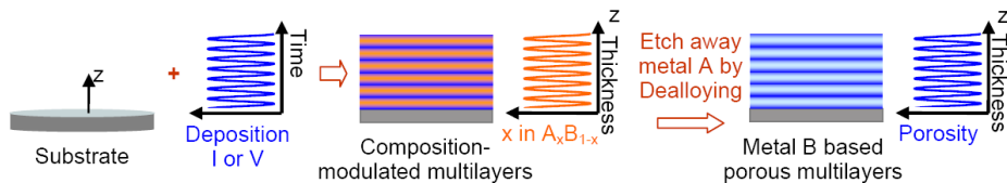
Figure 1. Fabrication of elaborate metallic films with modulated porosity along the thickness direction.
