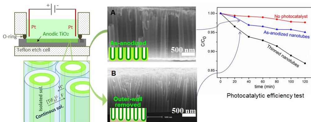
Figure 2. Selective removal of the outer shells of \text{TiO}_2 nanotubes for enhanced photocatalysis.
